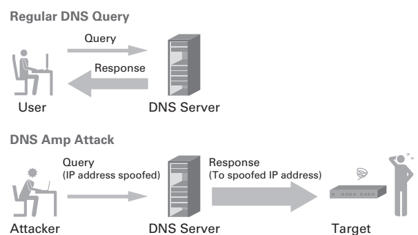
Figure 1: DNS Amp Attacks
