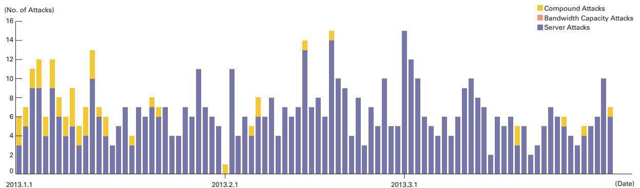
Figure 3: Trends in DDoS Attacks
